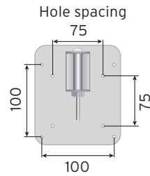
Screen plate
