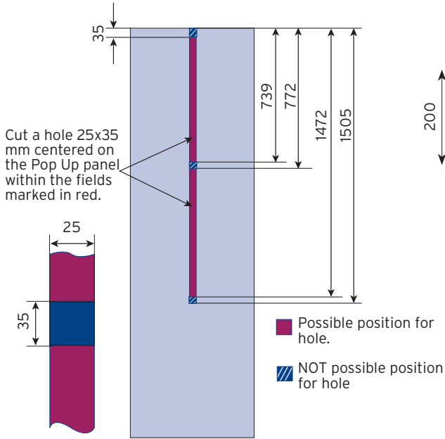
Position of holes in panel for Screen Holder/Shelf kit
