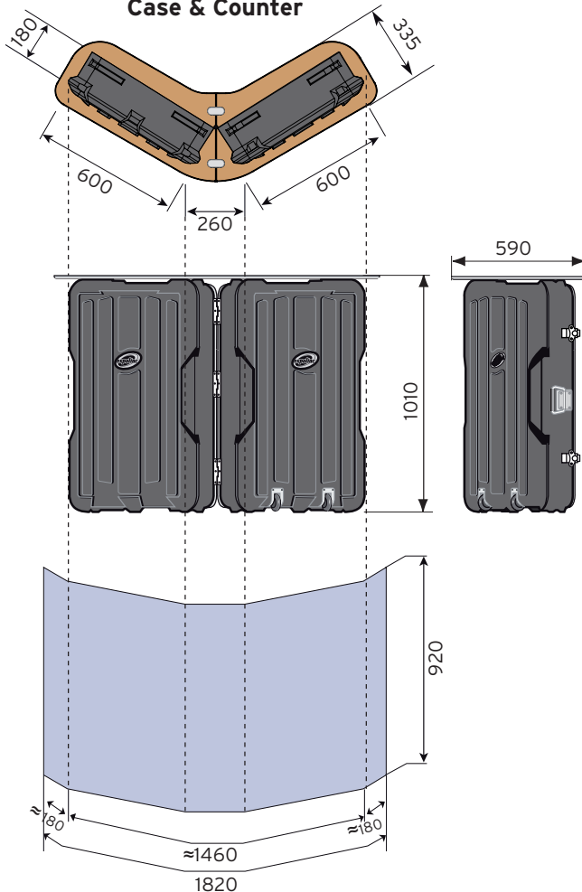
Case & Counter
